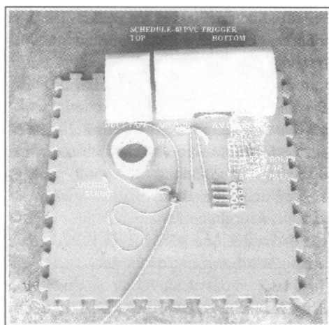
Fig. 1. Unassembled passive trigger designed to be used with the modified Aldrich foot snare for the capture of black bears.
