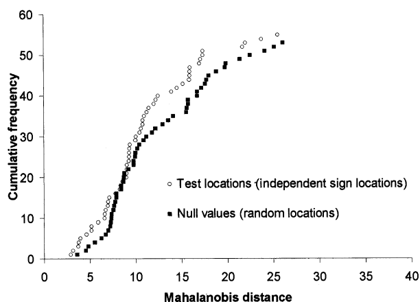
Fig. 5. Cumulative frequency of 61 independent bear sign and 61 random (null model) locations with associated Mahalanobis distance values, Oyacachi River Basin, Ecuador, 2000–01 for a study of Andean bear habitat use. Six outlying observations were excluded for scaling purposes.
