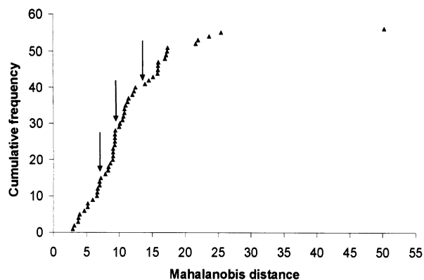
Fig. 4. Cumulative frequency of 61 test locations (independent locations of bear sign) and associated Mahalanobis distance values for a study of Andean bear habitat use in the Oyacachi River Basin, Ecuador, 2000–01. Four outlying observations were excluded for scaling purposes. Arrows indicate discontinuities used to define classes of Mahalanobis distance values.
