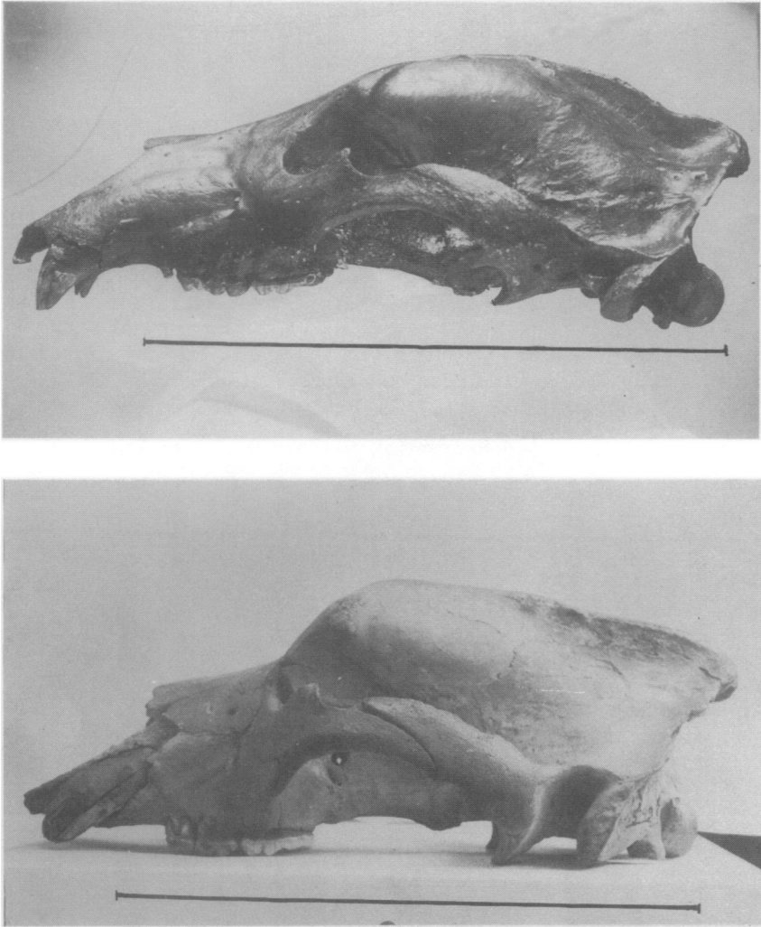
Fig. 4 Skulls of excavated bears: line indicates skull-length of modern brown bear. (a) Brown bear from the middle-fourth alluvium of the Volga River. (b) Large cave bear from the caves of the Zhigulevski heights.
