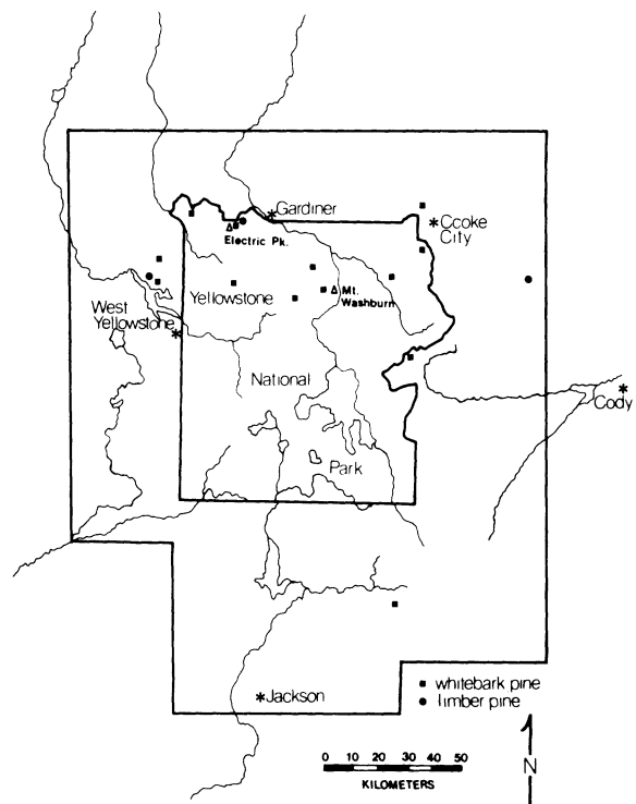
Fig. 1. Study area, including locations of 13 whitebark and 3 limber pine stands examined.
